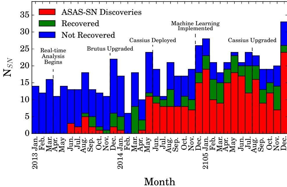
Figure 3. Histogram of bright supernovae discoveries in each month of 2013, 2014, and 2015. ASAS-SN discoveries are indicated in red, supernovae discovered by other sources and independently recovered by ASAS-SN are indicated in green, and supernovae that were not recovered by ASAS-SN are indicated in blue. Significant milestones in the ASAS-SN timeline are also indicated. The impact of ASAS-SN becoming operational in both hemispheres in 2014 May is clearly seen by a large increase in discoveries in all following months. ASAS-SN accounts for at least half of the bright supernova discoveries in every month after 2014 April, and also recovers a significant fraction of the supernovae it does not discover, particularly in 2015.
