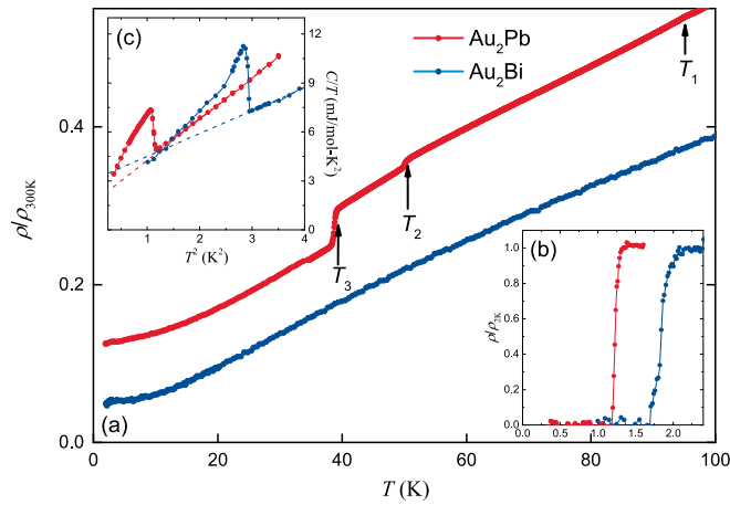
FIG. 2. (a) Cooling curves of the room temperature normalized electrical resistivity \rho/\rho_{300K} versus temperature T for Au_2Pb and Au_2Bi , where the structural transitions T_1 , T_2 , and T_3 in Au_2Pb are indicated by arrows. (b) Zoom of the normalized resistivity \rho/\rho_{2K} for T \leq 2.2 K, where superconductivity appears as sharp drops to zero resistivity. (c) Heat capacity divided by temperature C/T vs T^2 for Au_2Pb and Au_2Bi , where the superconducting transitions appear as sharp \lambda -type transitions. The dotted lines are fits to the data as described in the text.
