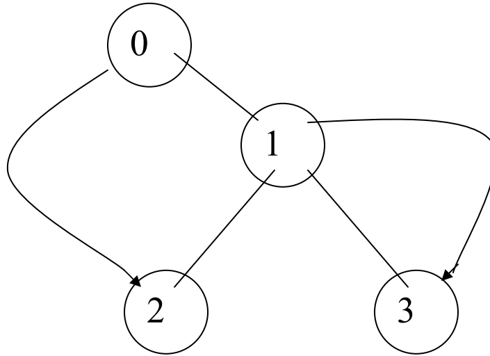
Figure 2.2 The binary spawn tree after spawn_rng is called on the node denoted by 0.
