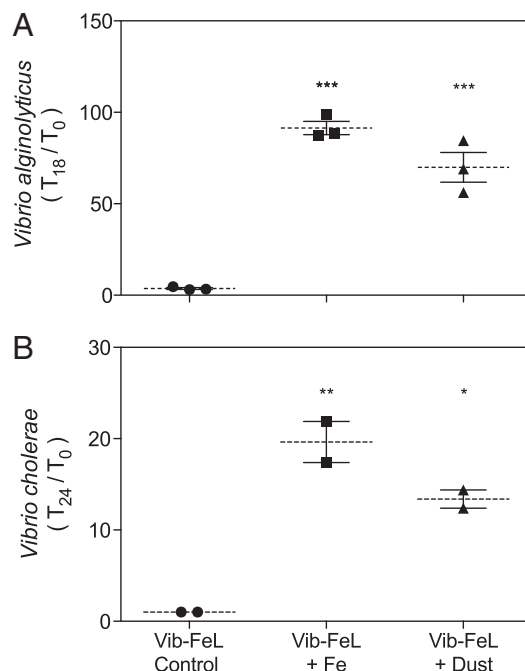
Fig. 2. Vibrio spp. response to Fe and dust. Growth of V. alginolyticus ( n = 3; A) and V. cholerae ( n = 2; B) in Fe-limited seawater (Vib-FeL) alone, amended with 4 \mu\text{M} FeCl 3 (Fe), and Dust SIM (Dust) containing 0.89 \mu\text{M} Fe. Vibrio growth was normalized among experiments by comparing the ratio of cfu·mL -1 after Dust SIM addition (T n ) to time 0 (T 0 ) (mean ± SEM). Asterisks indicate significantly greater growth with the addition of Fe and dust compared with growth in Vib-FeL alone (ANOVA). * P < 0.05; ** P < 0.01; *** P < 0.001. There was no significant difference between treatment with Dust SIM and treatment with Fe. Additional data are shown in Table S5.
